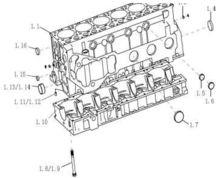
2. 1. 01 气缸总成/CYLINDER BLOCK
